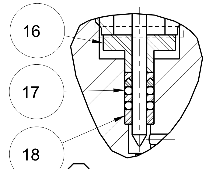
DETAIL A SCALE 2.000 60-11HF4-NO-212401
