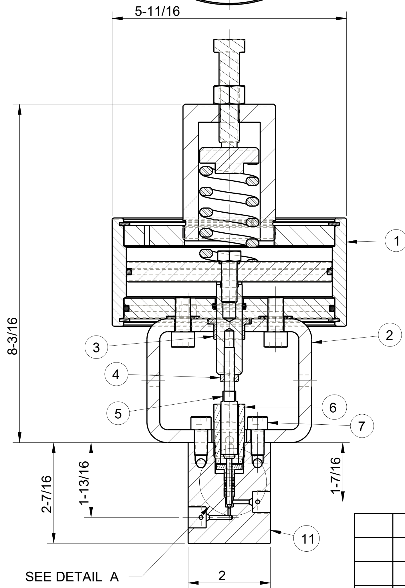
SECTION A-A SCALE 0.750
